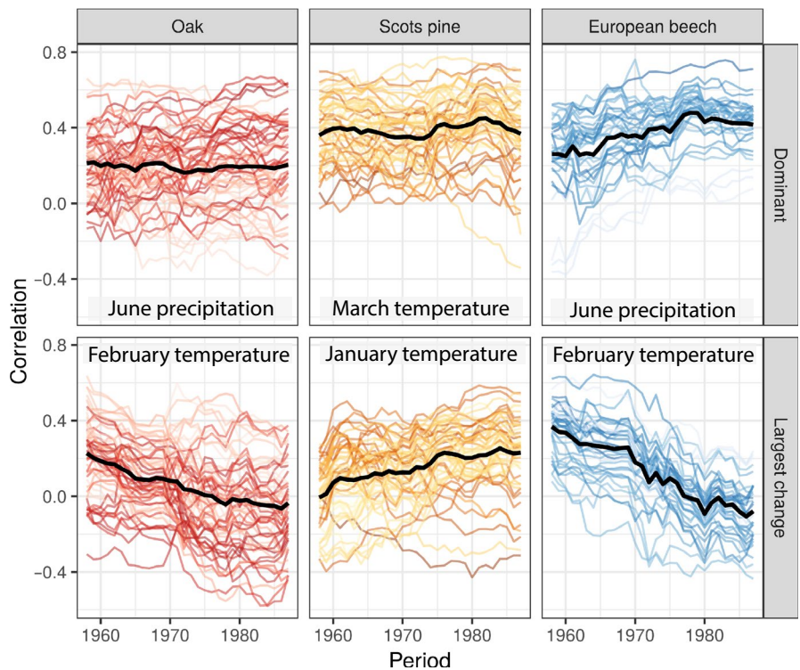
FIGURE 4 Results of moving correlation analysis estimating bootstrapped correlation values in 31 year moving windows offset by 1 year for each site included in the climate–growth analysis. Bootstrapped correlations for each site and each window are reported. The x-axis reports the last year of each 31 year window of analysis ('Period'). Colour shades were assigned based on the site longitude with dark (light) shades representing sites further west (east). Black lines represent mean bootstrapped correlation coefficients. The climate variables correlated to tree growth for each site are given in the inset text boxes
