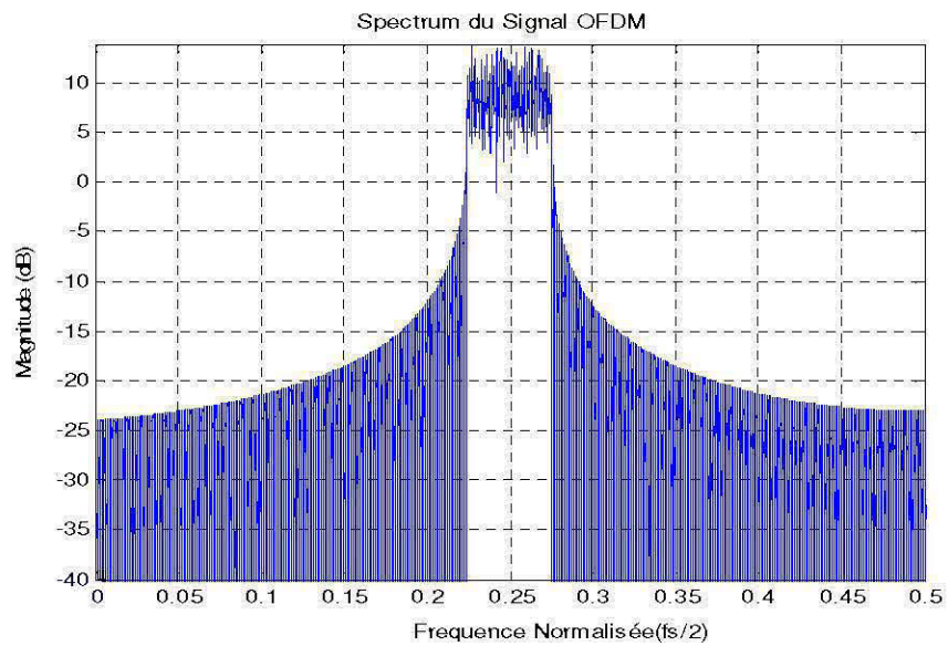
Figure 21 : Spectre de l'OFDM
