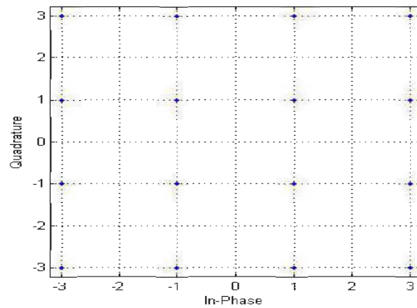
Figure 19 : Mappage 16-QAM
