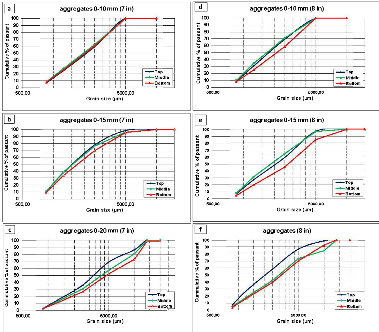
Figure 4.7 : Grain size distribution of cemented paste aggregate fill having 7 inches slump: a), b) and c), having 8 inches, d), e) and f)
