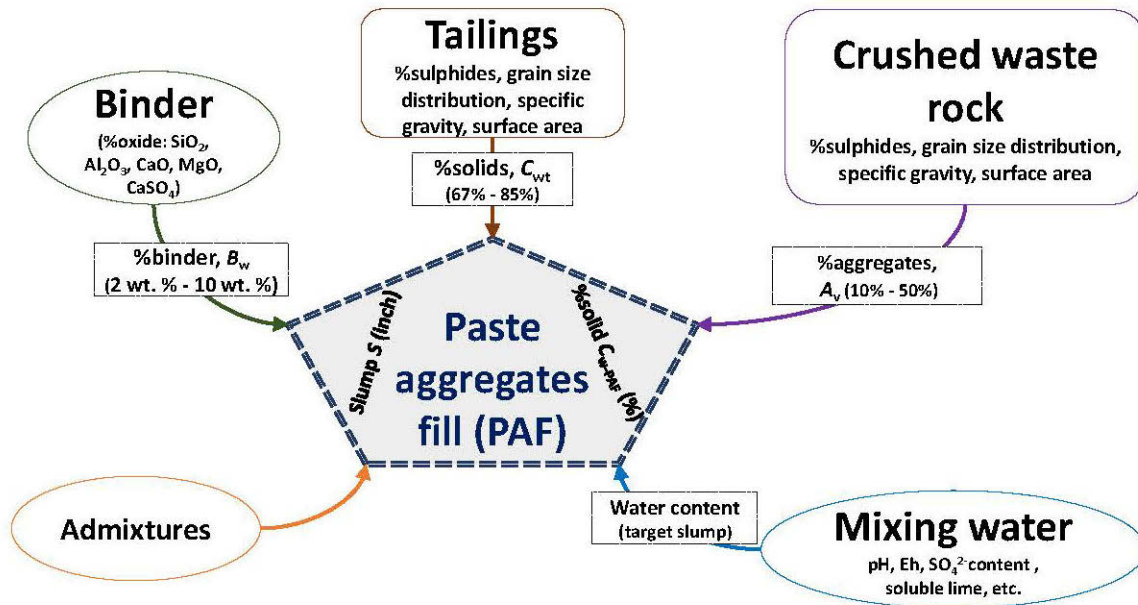
Figure 4.1 : Different components of PAF and the main factors that can affect their performance
