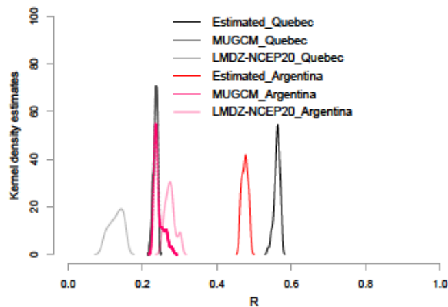
Figure 4. Density distributions of the coefficient of correlation ( R ) between observed and simulated \delta^{18}\text{O}_{\text{TR}} chronologies in Québec and Argentina when the simulations are based on \delta^{18}\text{O}_{\text{P}} series estimated by the regression model or from the MUGCM and LMDZ-NCEP20 models.
