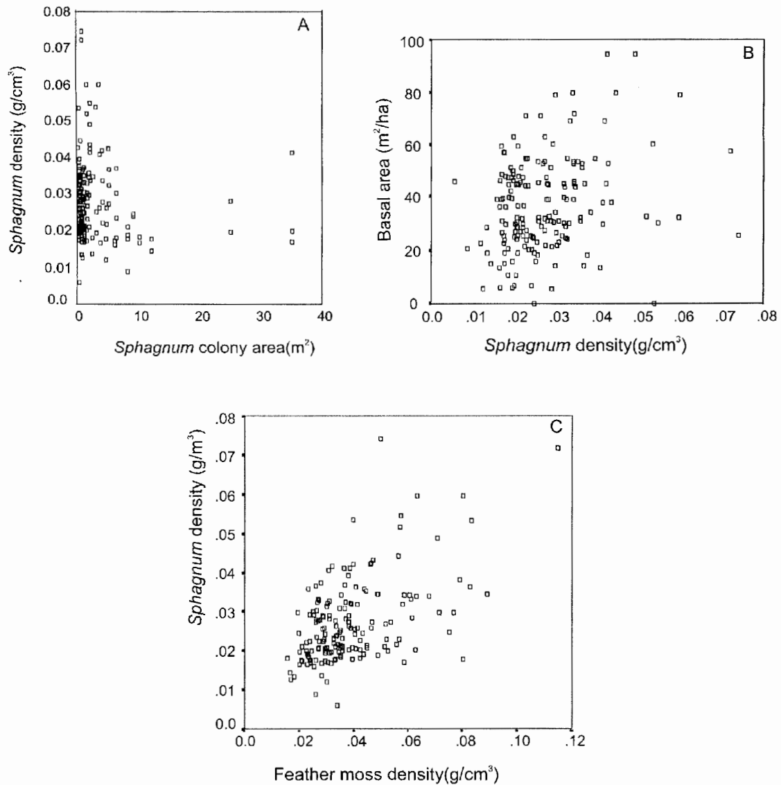
Figure 6.3 Relationships between Sphagnum colony density (g/cm 3 ) and (a) Sphagnum colony area (m 2 ), (b) tree basal area (m 2 /ha), and (c) feather mass density (g/cm 3 ).
