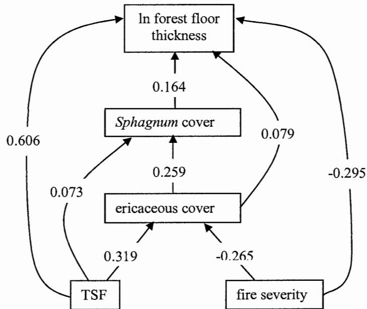
Figure 1.2 Path analysis of factors affecting forest floor thickness after high and low severity fires combined. The structure was not rejected by d-sep analysis (Shipley, 2000), p = 0.2989 . Multiple regression indicated that 70% of the variability was explained by the included variables. Arrows and numbers indicate the direction of causality and the path coefficient between two variables.
