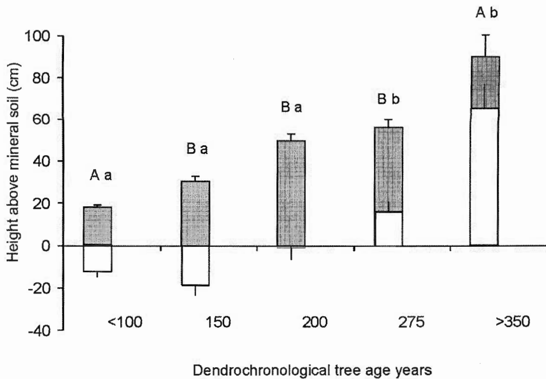
Figure 2.3 Changes in position of oxygen zone in soil profile with increasing tree age. Grey bars indicate the thickness of the organic forest floor, while white bars indicate the position of the oxygen zone (i.e. oxygen index). Letters indicate statistical differences, capital letters differences in oxygen zone thickness (relative to the profile surface), and lower case letters differences in the position of the oxygenated layer relative to the mineral soil – organic interface.
