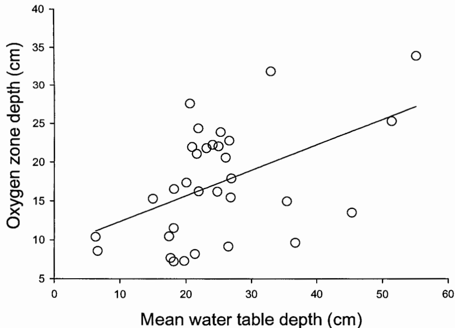
Figure 2.2 Relationship between oxygen zone depth and mean water table depth for the full sampling period (oxygen zone depth = 9.10 + 0.33 (mean water table depth), R^2 = 0.2325 , F value = 9.09, p = 0.0052 , N = 32 ).
