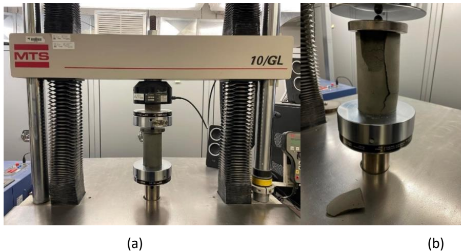
Figure 5 Uniaxial compression test: (a) Stiff mechanical press MTS 10/GL; (b) Broken sample after test
