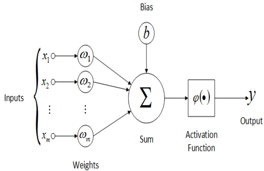
Figure 23: Presentation mathematical du RNA
