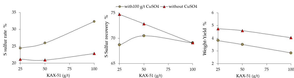
Figure 3. Yield weight and sulfur recovery during flotation tests (desulfurization).
